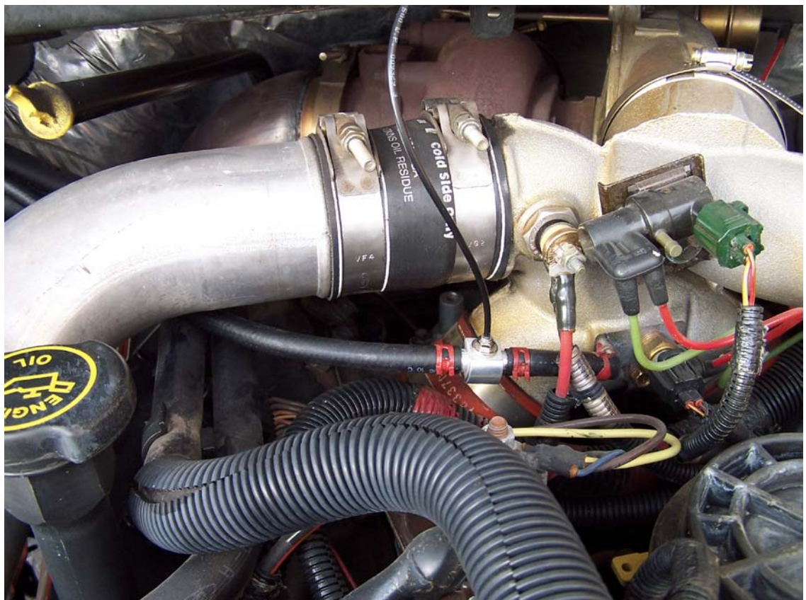
Figure 4 – Boost Gauge "T" Fitting Reinstalled
