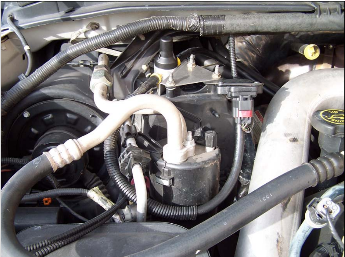
Figure 3 – Hose Routing from Overboost Annihilator to MAP Sensor
