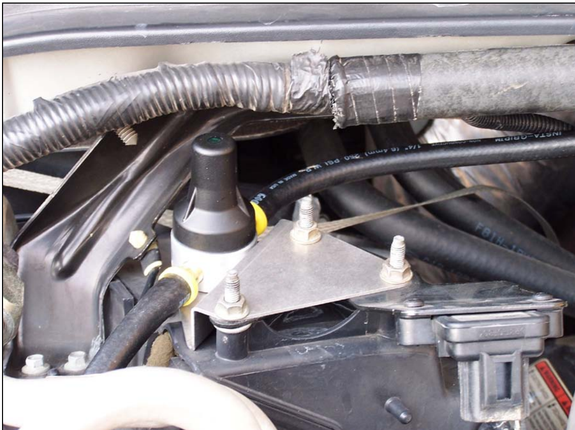
Figure 2 – Location of MAP Sensor Electrical Connector and Pressure Line
